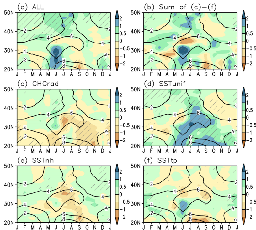
Figure 1. Sensitivity experiments with an AGCM showing time–latitude cross-sections of precipitation (shading; \text{mm day}^{-1} ) averaged over 125^{\circ}\text{E}–145^{\circ}\text{E} . (a) RCP8.5 scenario, (b) sum of (c)–(f), (c) greenhouse-gas radiative forcing, (d) uniform SST warming, (e) SST pattern change in the Northern Hemisphere extratropics, (f) SST pattern change in the tropics. Contours indicate the present-day climatology. Hatching indicates that the change is statistically significant.
