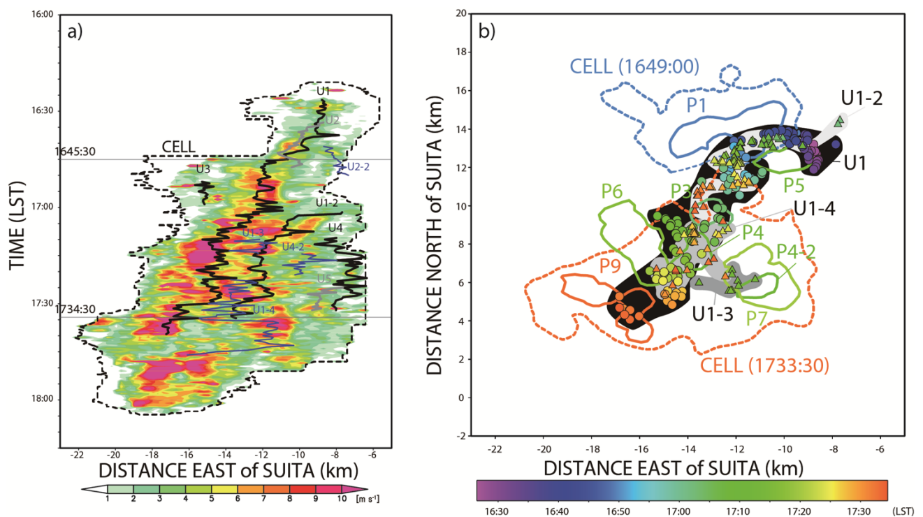
Figure 1. (a) Time–distance cross-section of the maximum updraft at 2 km above sea level (ASL) within the north–south range of the cell. The black, gray, and blue lines indicate the center of the identified updraft cores. The dashed line indicates the easternmost and westernmost edges of the cell. (b) Location of the precipitation core (bold lines) and cell (dashed lines) at 6 km ASL, and the centers of the updraft cores (circles and triangles) at 2 km ASL. The black and gray areas represent regions where the center of each updraft core passed through.
