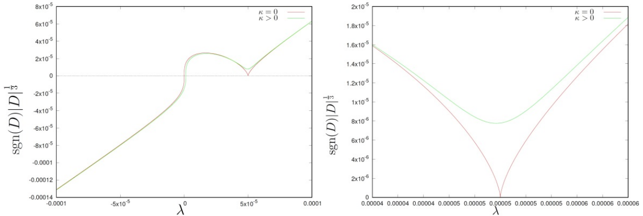
Figure 1: Graphs of \text{sgn}(D)|D|^{1/3} for \kappa = \frac{f\pi}{NH} = 0 \text{ m}^{-1} (red) and \kappa = \frac{f\pi}{NH} = 2 \times 10^{-6} \text{ m}^{-1} (green) as functions of \lambda , where f is the Coriolis parameter, H is the fluid depth, and N is the reference buoyancy frequency. An enlarged view in the vicinity of multiple root for \kappa = 0 is shown at the right. The parameter values are set such that the linear growth condition is satisfied.
