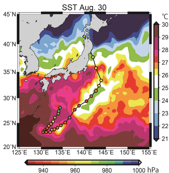
← Figure 1. Horizontal distribution of TRMM/TMI daily mean SST on 30 August 2016. Colors indicate water temperature ( ^{\circ}\text{C} ). Circles indicate the location and central pressure of Typhoon Lionrock.
