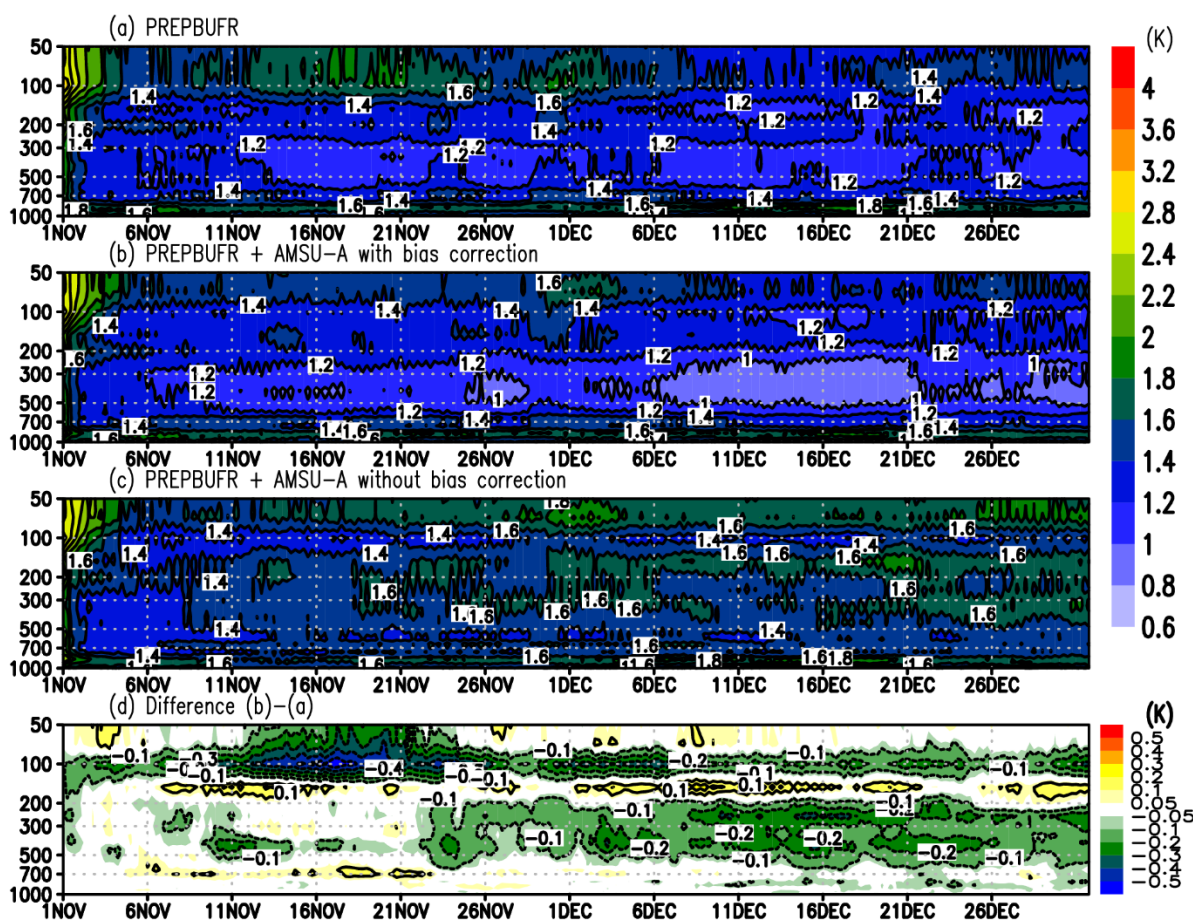
Figure 1. Time series of the globally-averaged root mean square differences (RMSD) for temperature (K) relative to the ERA-Interim for the experiments (a) with PREPBUFR only, (b, c) with additional AMSU-A with and without bias corrections, respectively. (d) shows the difference between (a) and (b), with negative values corresponding to the advantage by assimilating the AMSU-A radiances. The horizontal and vertical axes represent the date and pressure level, respectively.
